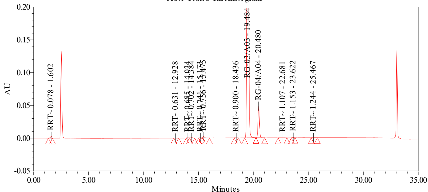
Auto-Scaled Chromatogram
